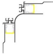
Plaster Board Cornice LED Channel ~ Model Alu-Cove3
