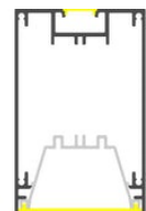
3.5x2.2" Linear Suspension Lighting Channel ~ Model Munich Magnum
