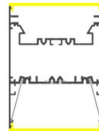
Direct/Indirect Linear Pendant Lighting LED Channel ~ Model DPL70FL
